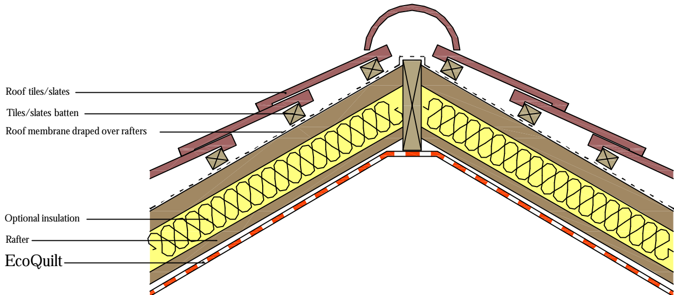
Additional Attic Insulation - Pitch Detail
