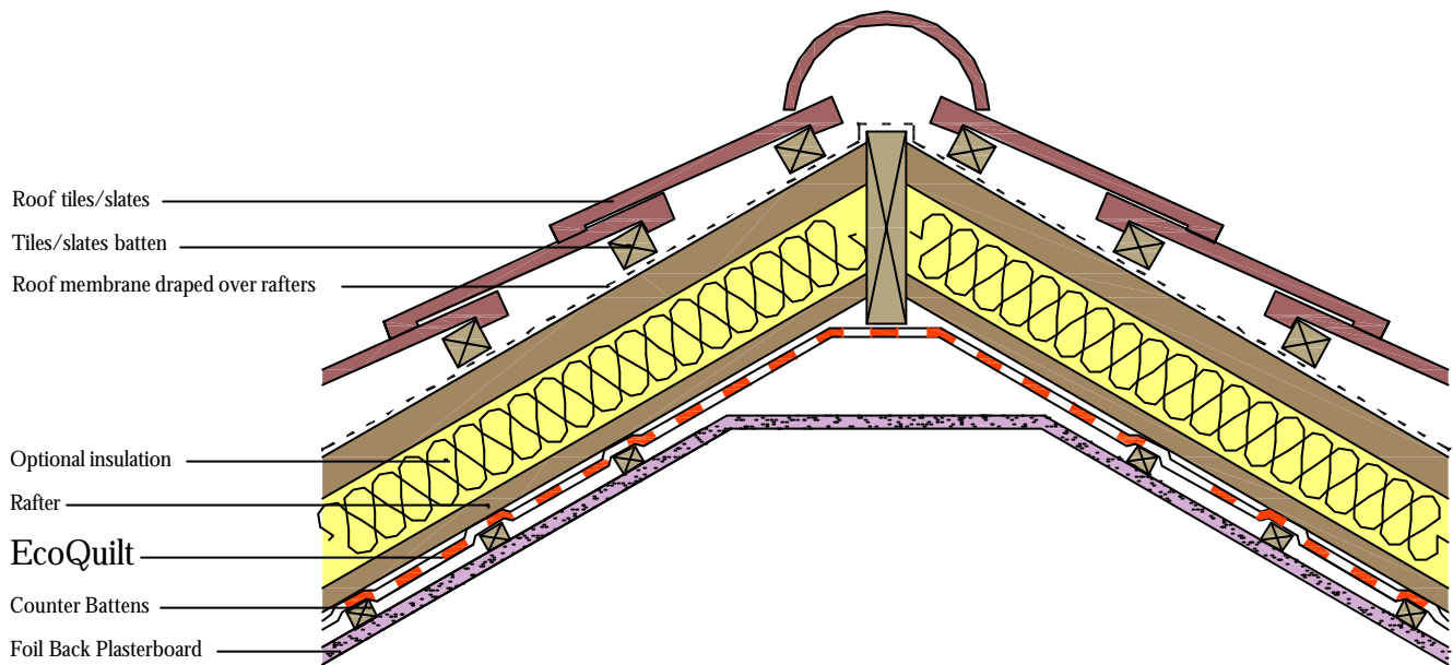
Attic Conversion - Pitch Detail
