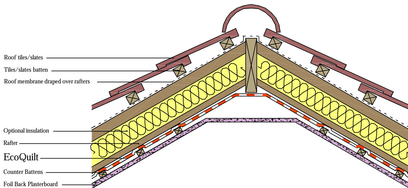
Attic Conversion - Pitch Detail
