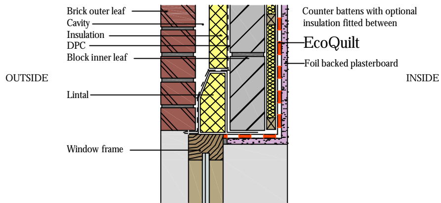
Window Head Detail
