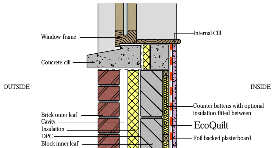
Window Cill Detail
