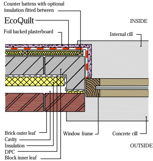
Window Jamb Detail
